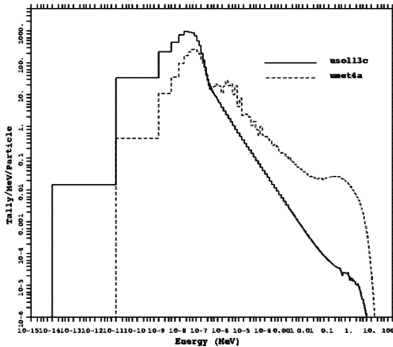
Figure 1: Comparison of Neutron Flux Spectra for USOL13C and UMET4A.
